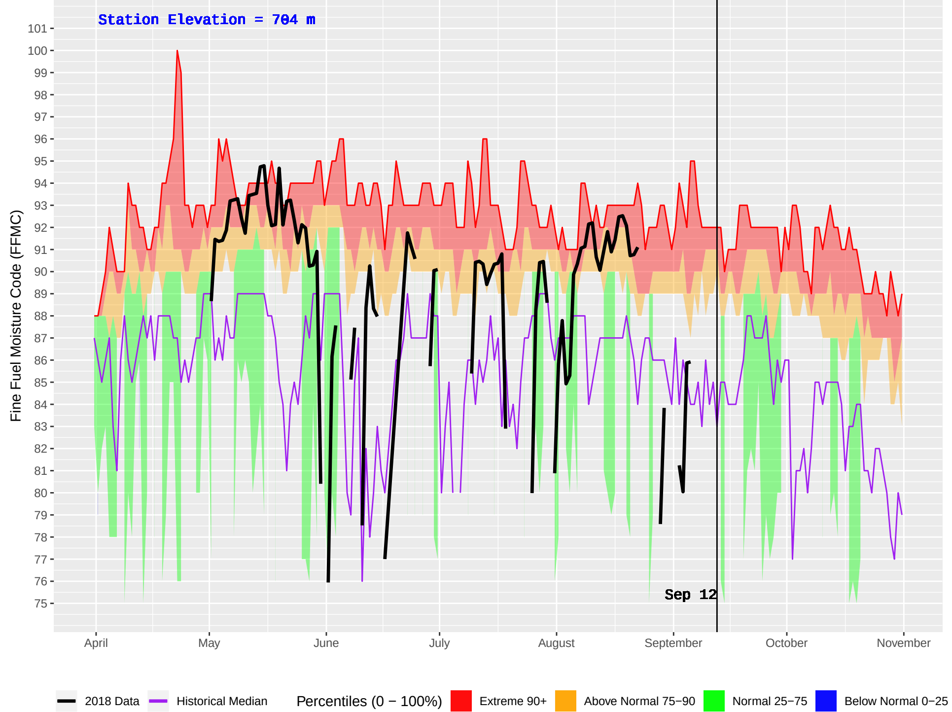
HUDSON HOPE (132) : Historical (1986–2016) and Current (2018) Daily Fine Fuel Moisture Code (FFMC)
