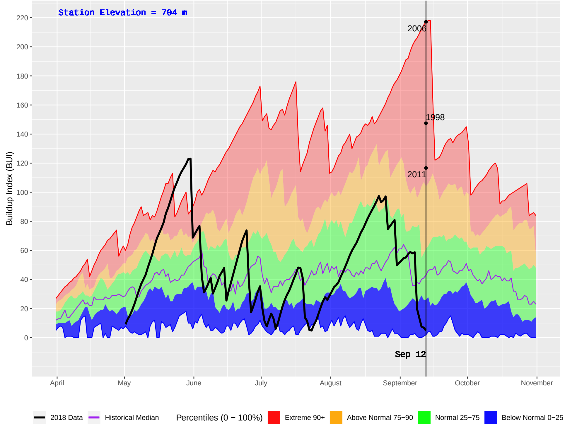
HUDSON HOPE (132) : Historical (1986–2016) and Current (2018) Daily Buildup Index (BUI)
