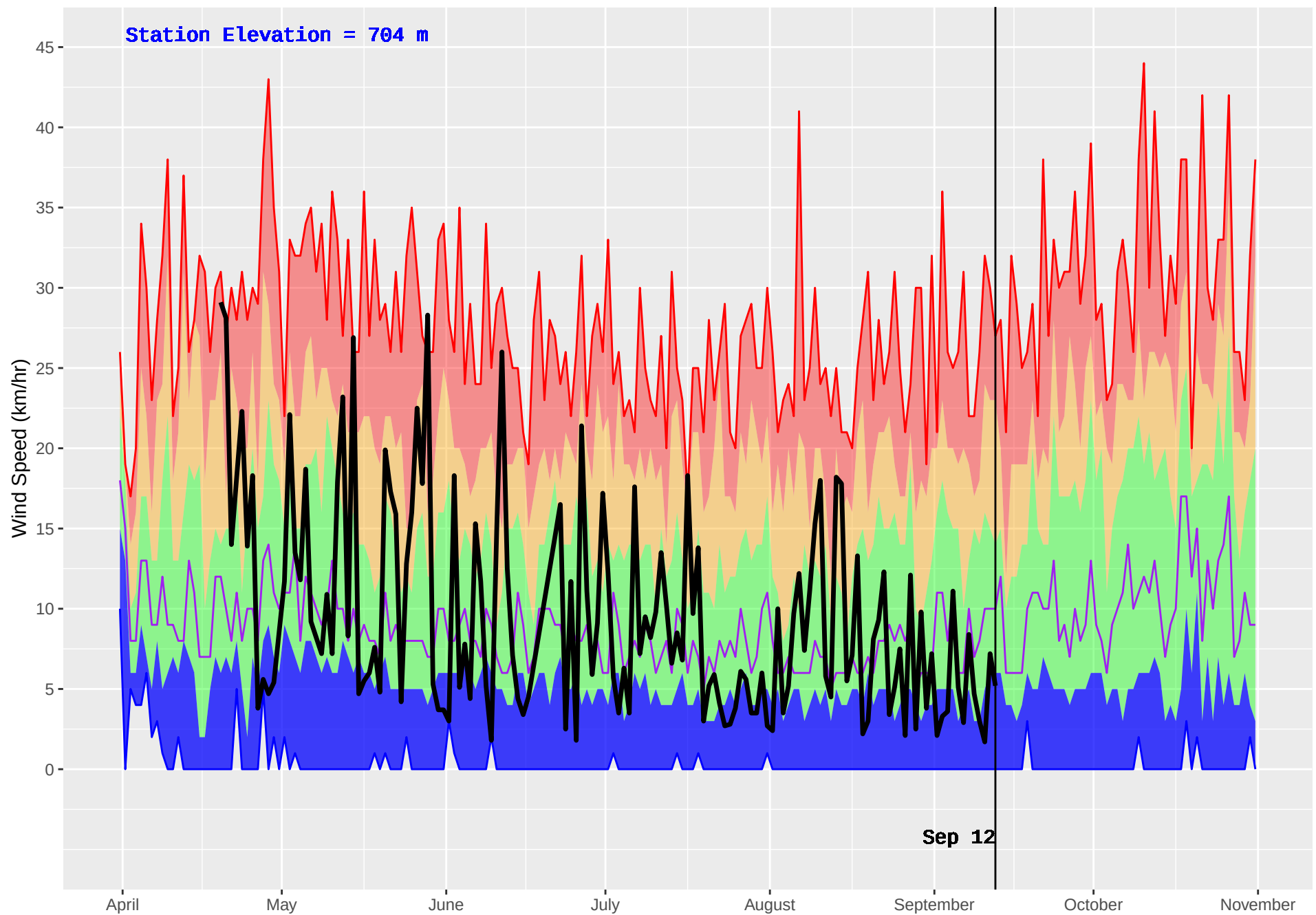
HUDSON HOPE (132) : Historical (1986–2016) and Current (2018) Daily Wind Speed
